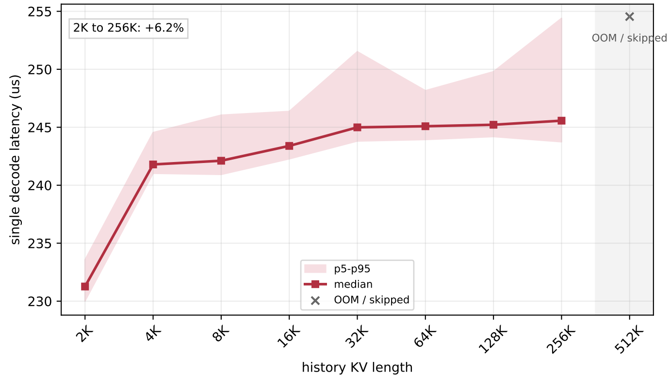
H800 FlashMLA sparse FP8 decode latency - batch=256
