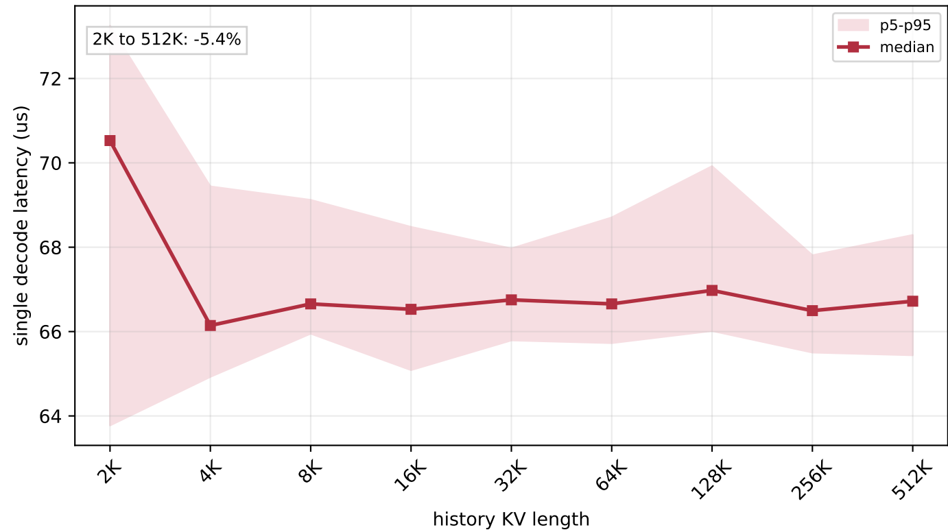
H800 FlashMLA sparse FP8 decode latency - batch=32
