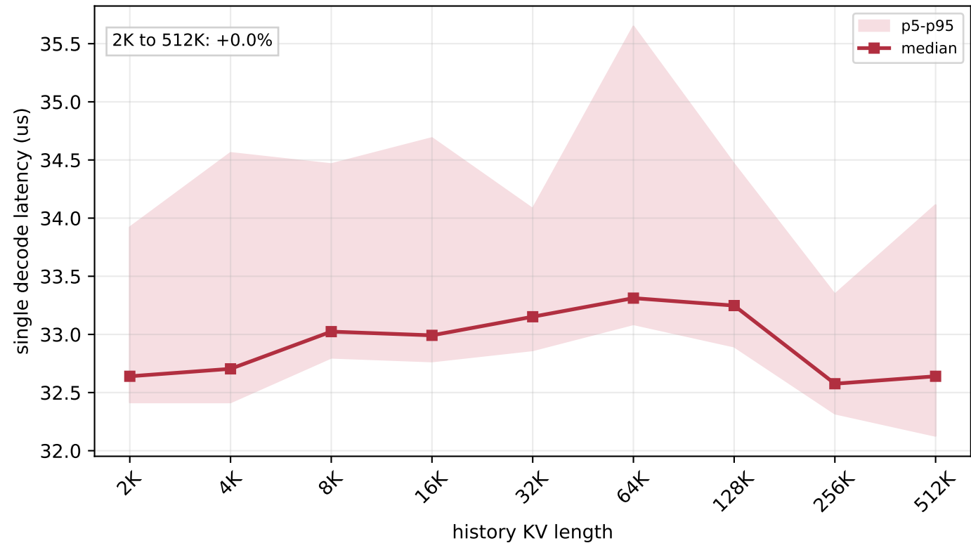
H800 FlashMLA sparse FP8 decode latency - batch=4
