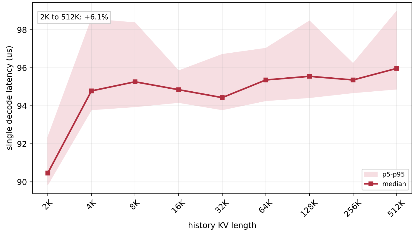
H800 FlashMLA sparse FP8 decode latency - batch=64
