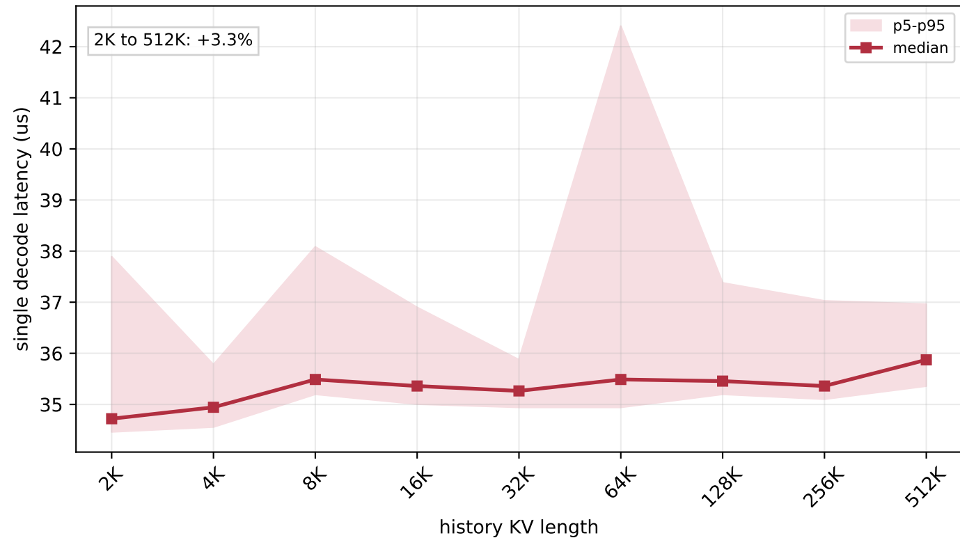
H800 FlashMLA sparse FP8 decode latency - batch=8
