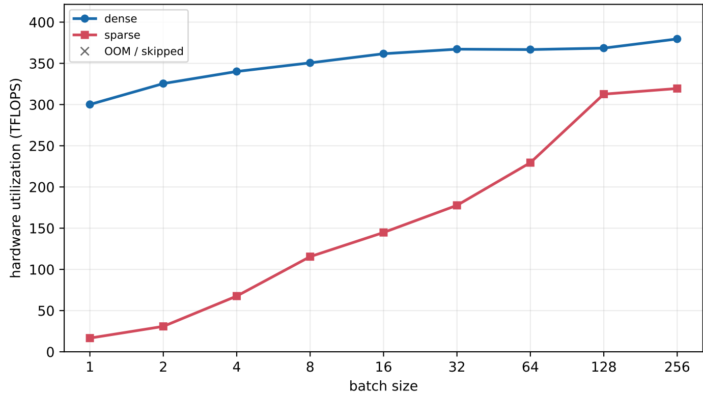
H800 MLA - H=128K, Q=1 (decode)
