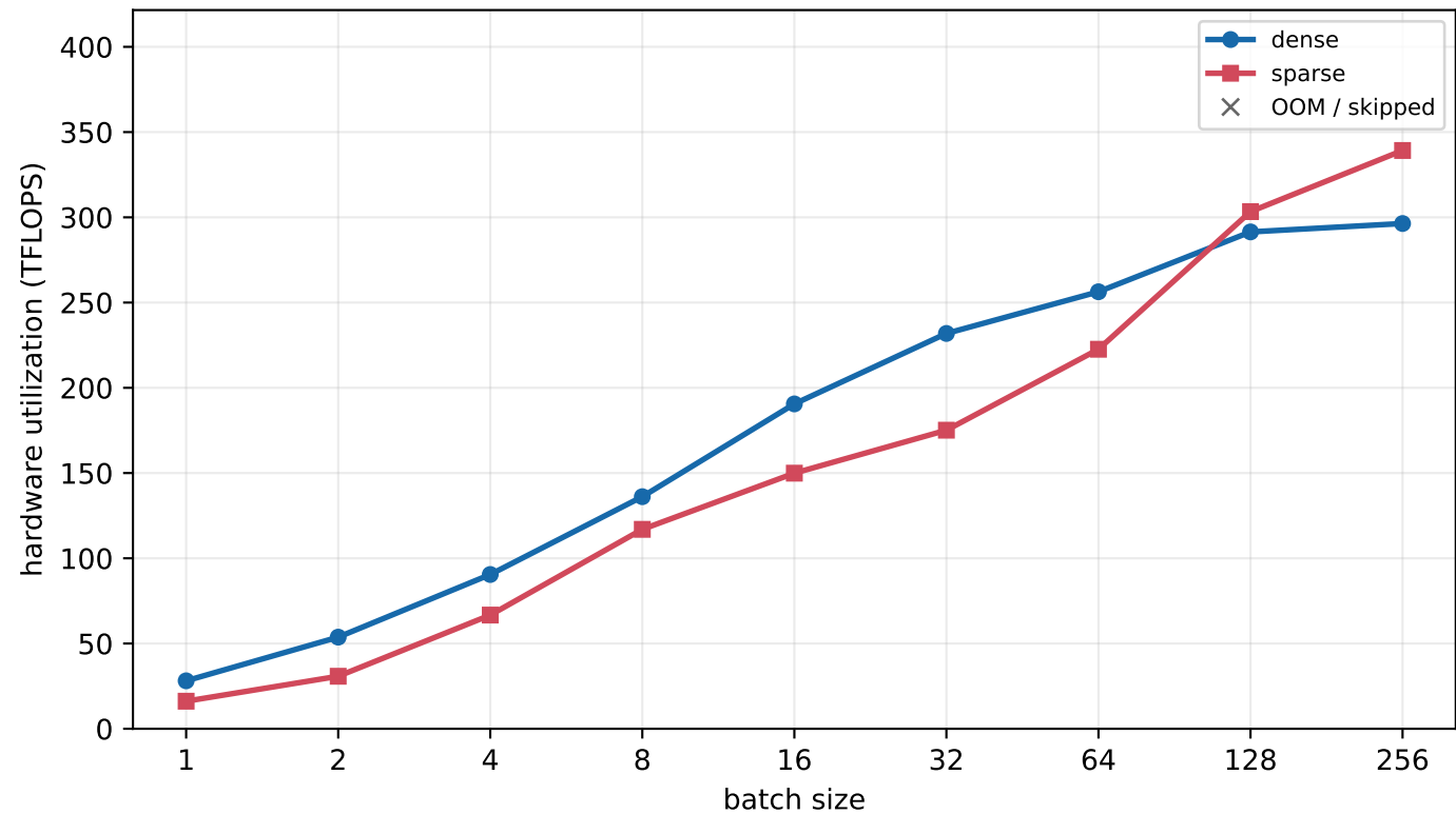
H800 MLA - H=2K, Q=1 (decode)
