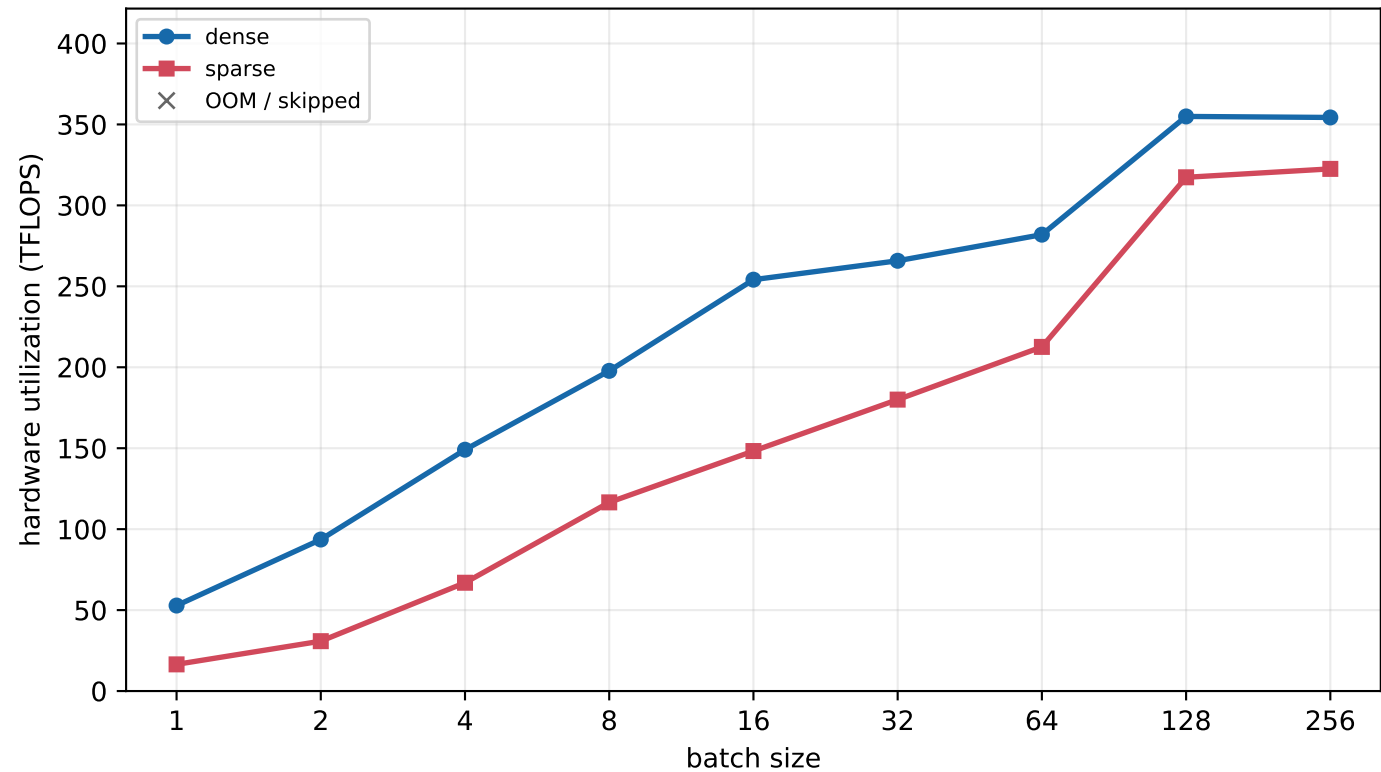
H800 MLA - H=4K, Q=1 (decode)
