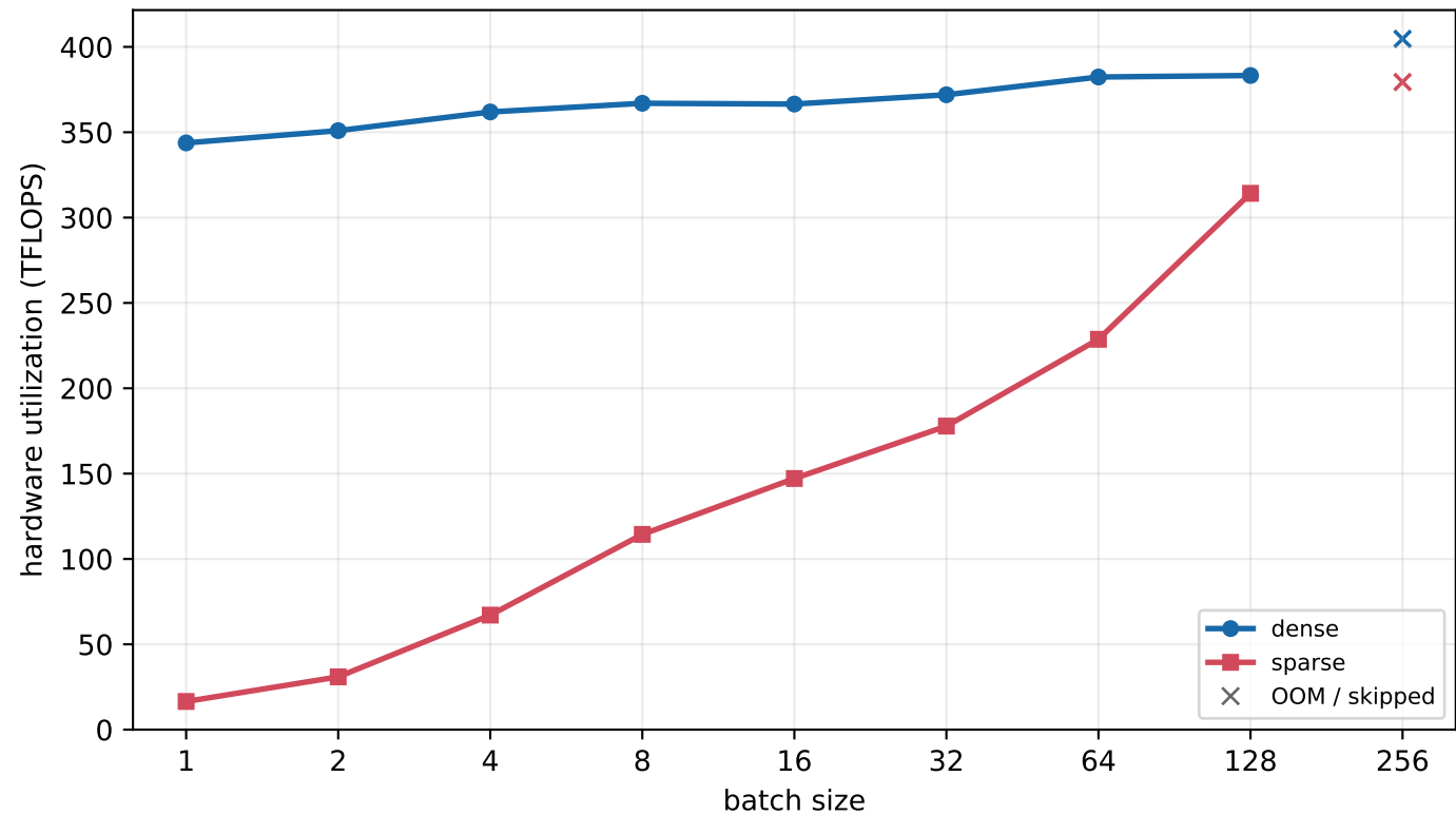
H800 MLA - H=512K, Q=1 (decode)
