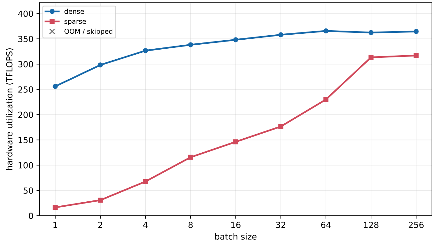
H800 MLA - H=64K, Q=1 (decode)
