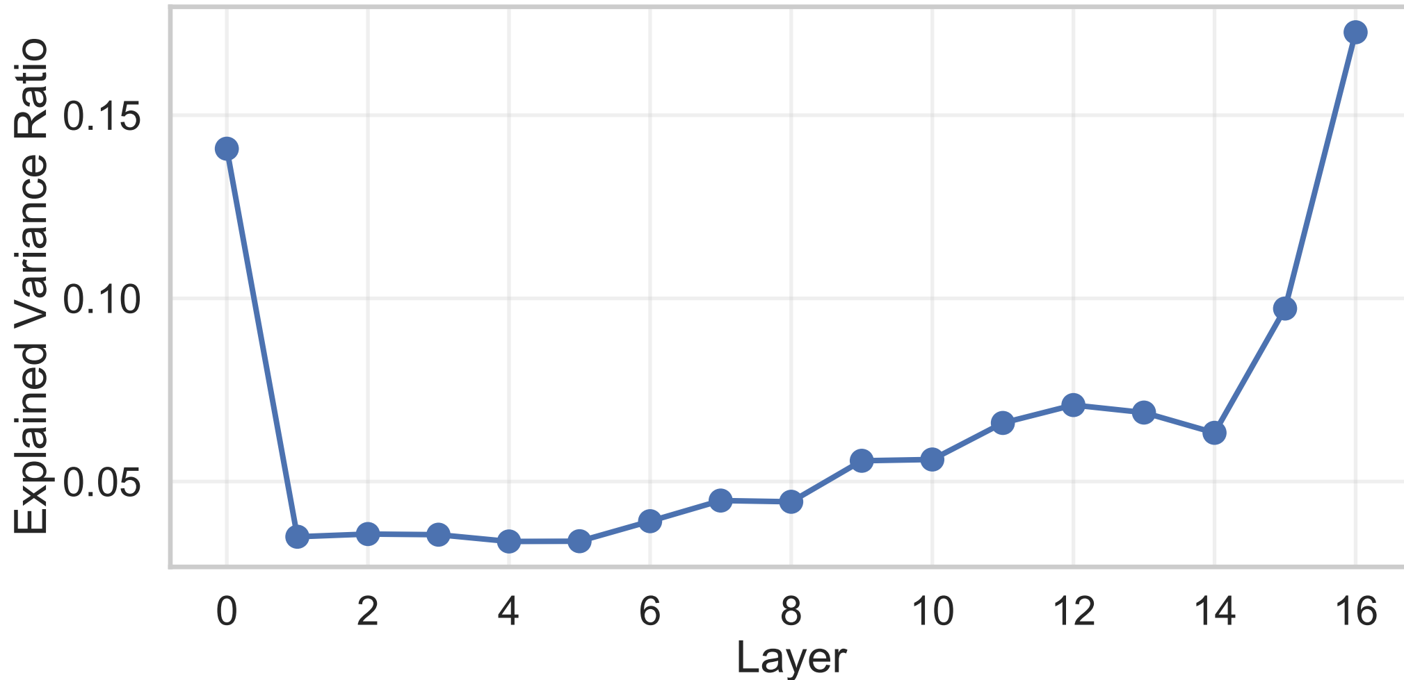
—●— Explained variance for 1st PCA component
