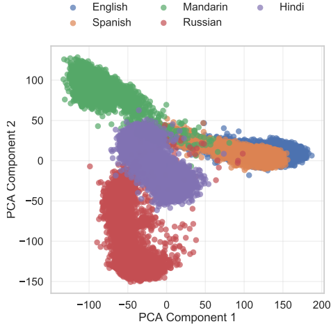
(a) Final layer language map (Qwen)
