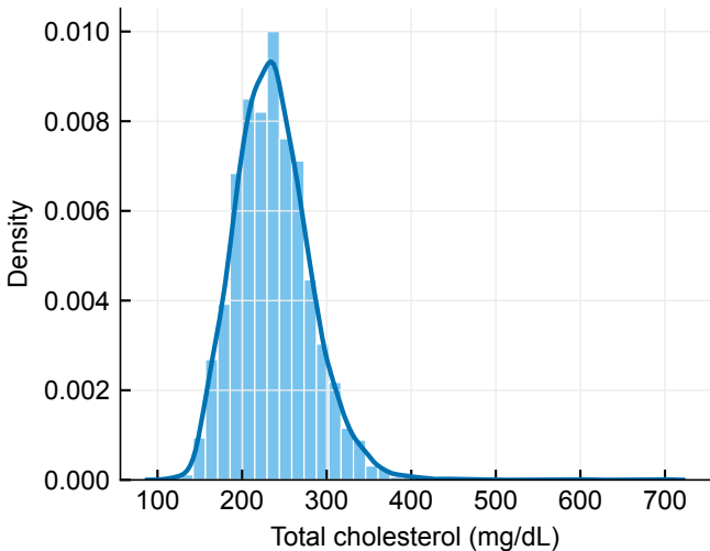
Distribution of total cholesterol (baseline)
