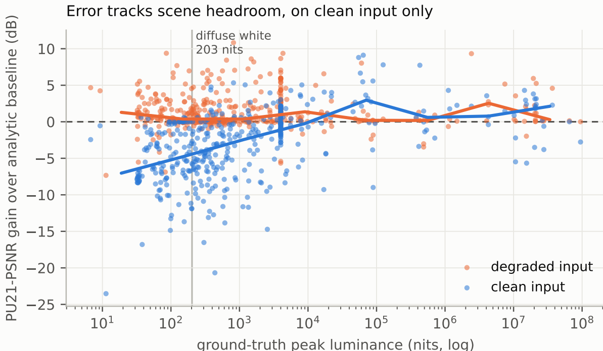
Figure 2. Per-frame gain against the headroom the ground truth actually has, log x-axis, with binned medians. On clean input the trend rises through zero at roughly 10,000 nits; on degraded input it is flat and positive at every headroom. The model’s error is a function of the scene, and only when the input arrives clean.
