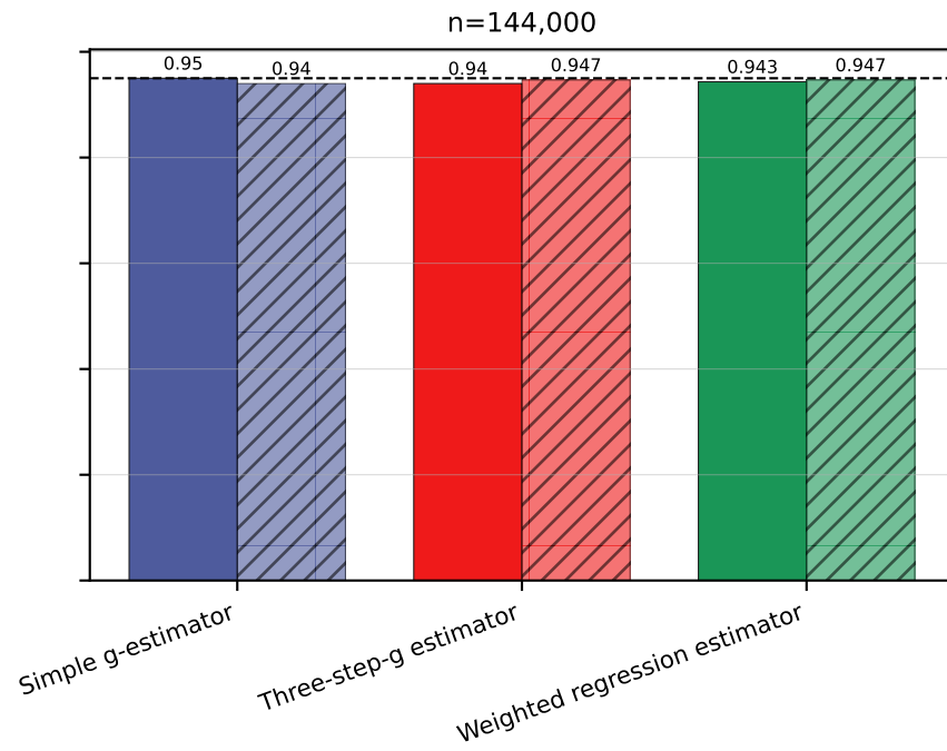
Empirical coverage of \psi_{05} at the hard cell — Oracle vs Super-learner nuisances
