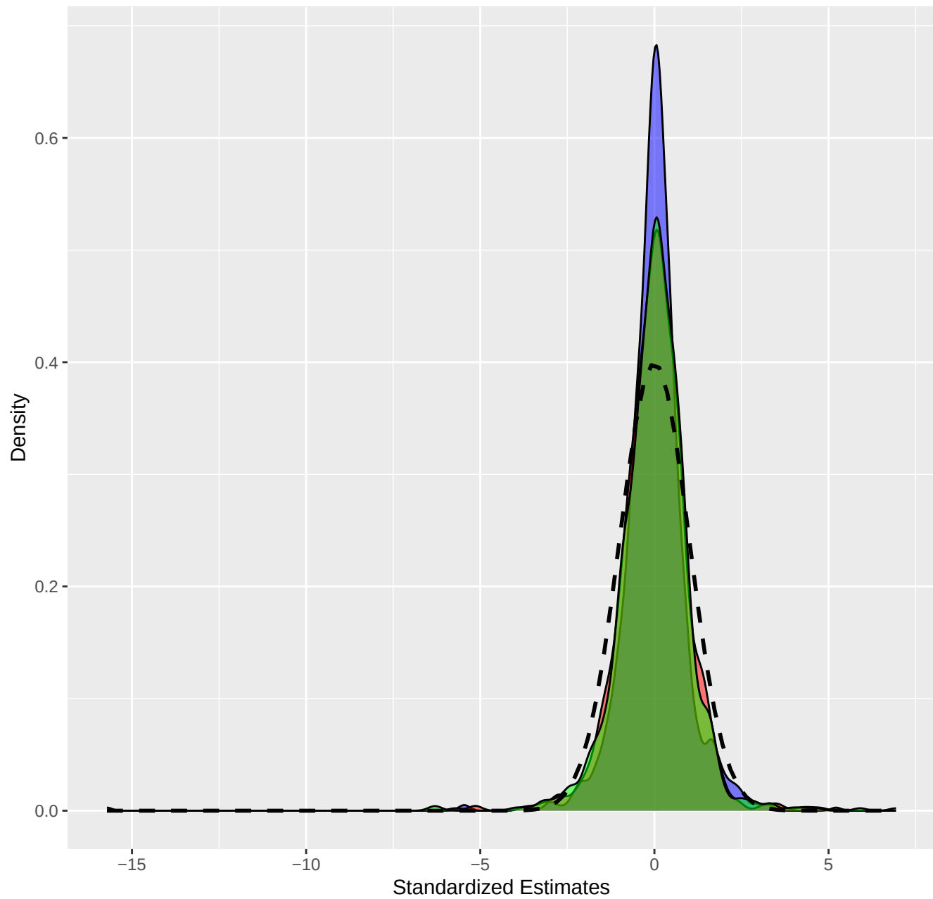
Density Plot of Standardized Estimates for psi03
