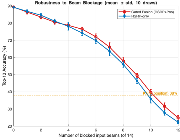
Fig. 2. Top- K accuracy ( K=13 ) vs. number of blocked input beams; error bars are \pm 1 standard deviation over 10 blockage draws. The gated fusion matches RSRP-only when clean and improves it under blockage; KNN (position only) is flat.
