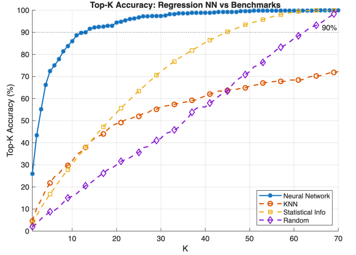
Fig. 1. Reproduced benchmark: top- K accuracy of the RSRP-regression network vs. KNN, Statistical, and Random baselines. The network reaches 90% at K = 13 .
