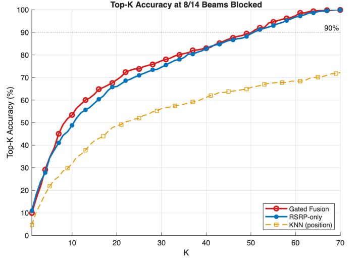
Fig. 3. Top- K accuracy vs. K at a representative 8/14 blocked input beams. The gated fusion dominates the RSRP-only model across K ; both far exceed position-only KNN.
