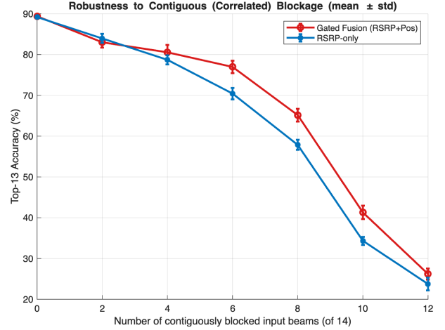
Fig. 5. Additional robustness study: top- K accuracy ( K=13 ) under contiguous (correlated) blockage of the sampled beams; error bars are \pm 1 std over 10 draws. The gated-fusion advantage over RSRP-only is larger than under i.i.d. blockage (cf. Fig. 2).
