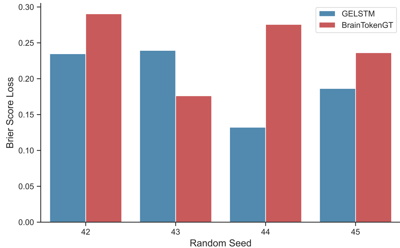
B. Brier Score by Seed (Lower is Better) GELSTM Mean: 0.1982 vs. BrainTokenGT: 0.2446
