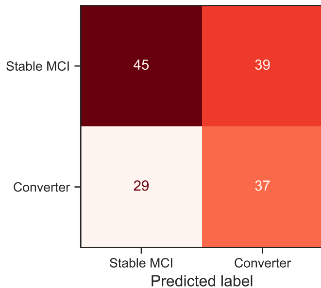
BrainTokenGT (Seed 42, 6 runs pooled) mean F1=0.509
