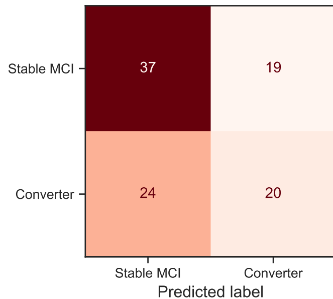
BrainTokenGT (Seed 43, 4 runs pooled) mean F1=0.448
