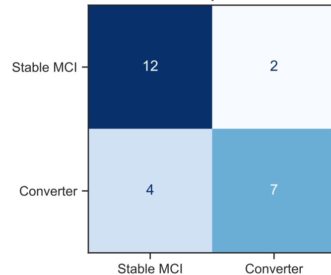
BrainTokenGT (Seed 45, 4 runs pooled) mean F1=0.560
