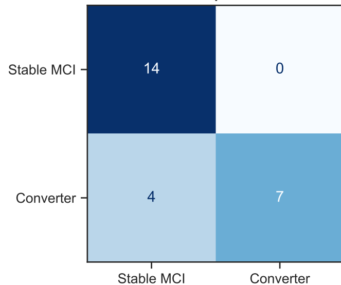
BrainTokenGT (Seed 43, 4 runs pooled) mean F1=0.448
