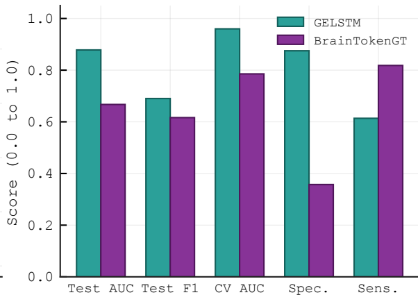
B. Multi-Metric Comparison Profile
