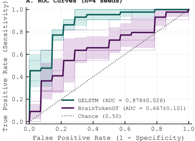
A. ROC Curves (n=4 seeds)
