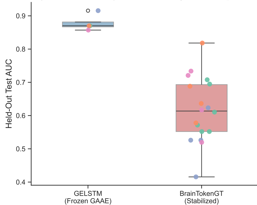
B. Held-Out Test AUC — GELSTM (n=4) vs BrainTokenGT (n=18) Wilcoxon (seed-paired, n=4) p=0.1250; margin 95% CI [+0.157, +0.375]
