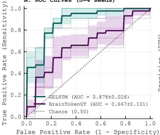
A. ROC Curves (n=4 seeds)
