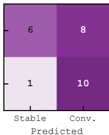
BrainTokenGT (Seed 43) Th=0.29 | F1=0.69
