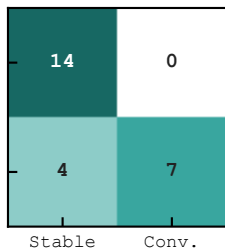
BrainTokenGT (Seed 43) Th=0.29 | F1=0.69
