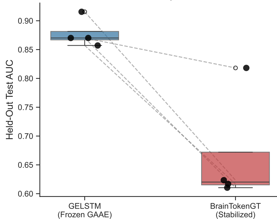
B. Held-Out Test AUC (n=4 seeds) Paired t=3.90 , p=0.0299 *
