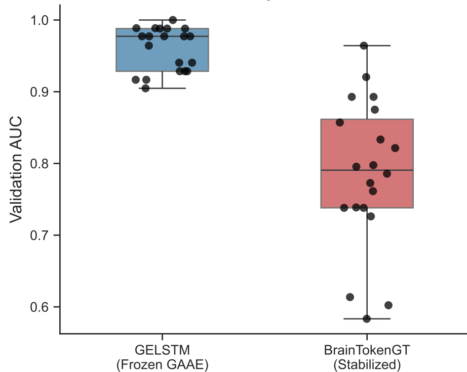
A. 5-Fold CV AUC Distribution (n=20 folds) Paired t=6.84 , p=1.59\text{e-}06 ***
