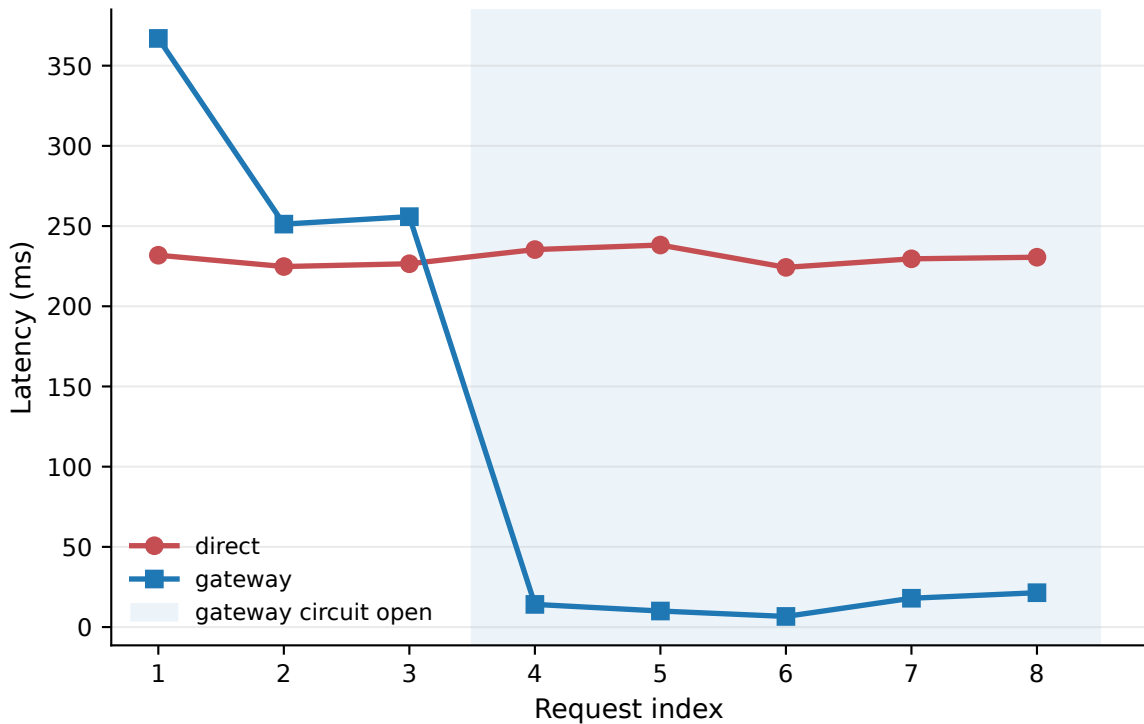
Circuit breaker: fail-fast after threshold
