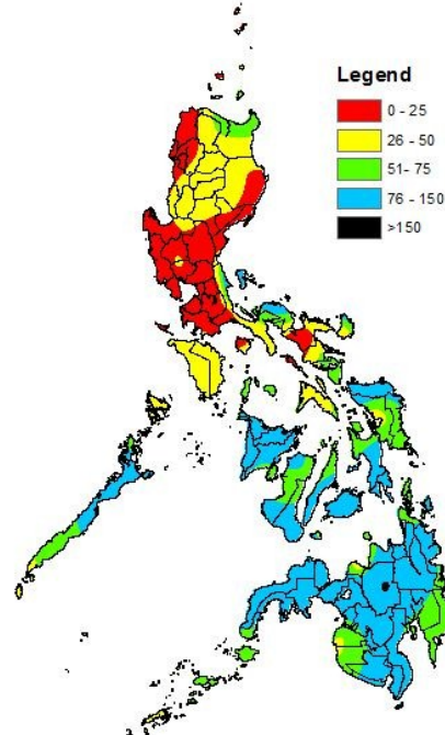
Ten-day Regional Rainfall Forecast (mm) November 1 - 10, 2016 Decade 31
