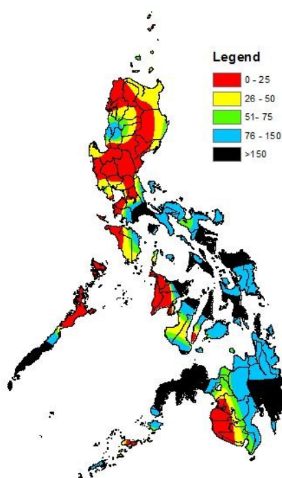
Actual Rainfall Distribution (mm) October 21 - 31, 2016 Decade 30
