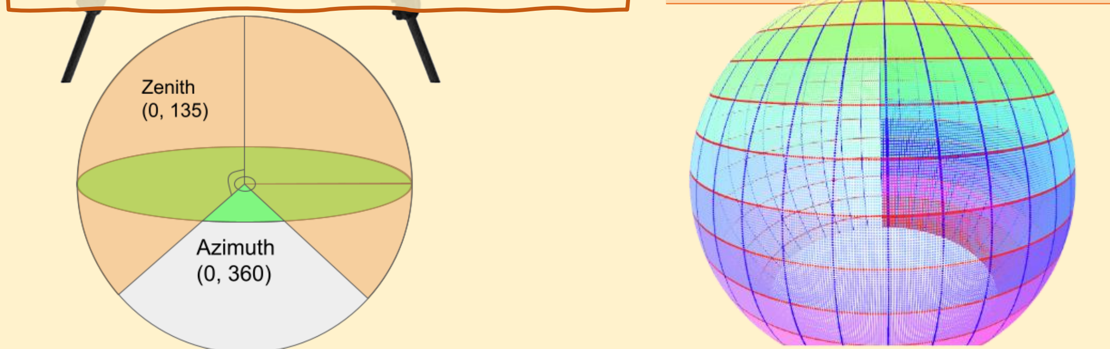
Field of View of the CBL LiDAR. Scan Pattern Projected onto a 3D Sphere.
