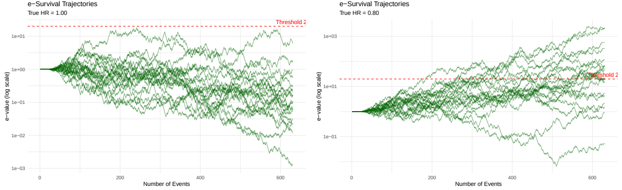
Figure 8: Trajectories of the fixed-magnitude e-RTs process for a trial designed to detect a Hazard Ratio of 0.80 with 80% fixed-sample log-rank power (631 events). Left: trajectories under the null hypothesis ( HR = 1.00 ), where wealth fluctuates randomly. Right: trajectories under the alternative hypothesis ( HR = 0.80 ), where wealth grows systematically. The red dashed line represents the rejection threshold ( 1/\alpha = 20 ).
