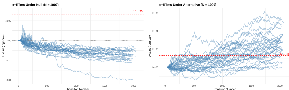
Figure 9: Trajectories of e-RTms for a trial with N = 1000 patients. Left: under the null hypothesis (equal transition matrices), wealth fluctuates randomly. Right: under the alternative hypothesis, wealth grows as treatment improves recovery transitions. Dashed red line: rejection threshold ( 1/\alpha = 20 ).
