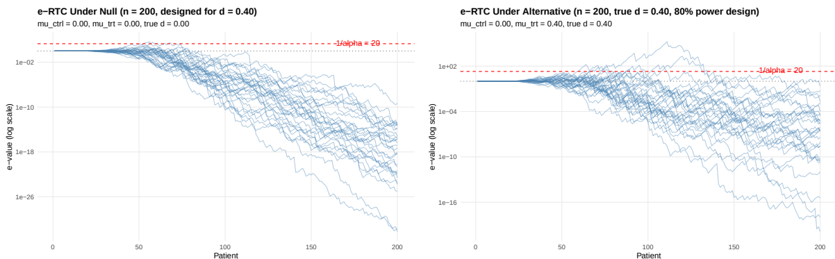
Figure 7: Trajectories of the continuous randomization e-process for a trial designed to detect a standardized mean difference of d = 0.40 with 80% power. Left: trajectories under the null hypothesis ( d = 0 ), where wealth wanders near or below 1 and rarely approaches the rejection threshold ( 1/\alpha = 20 ). Right: trajectories under the alternative hypothesis ( d = 0.40 ), where wealth grows systematically and many paths cross the rejection threshold before the planned sample size is reached.
