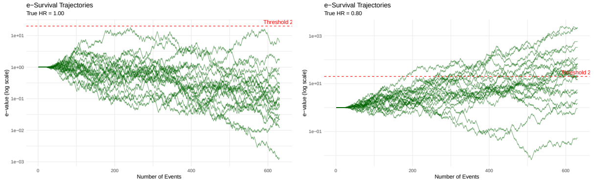
Figure 10: Trajectories of the fixed-magnitude e-RTs process for a trial designed to detect a Hazard Ratio of 0.80 with 80% fixed-sample log-rank power (631 events). Left: trajectories under the null hypothesis ( \text{HR} = 1.00 ), where wealth fluctuates randomly. Right: trajectories under the alternative hypothesis ( \text{HR} = 0.80 ), where wealth grows systematically. The red dashed line represents the rejection threshold ( 1/\alpha = 20 ).
