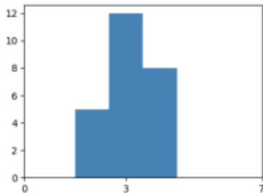
Histograma — Original
