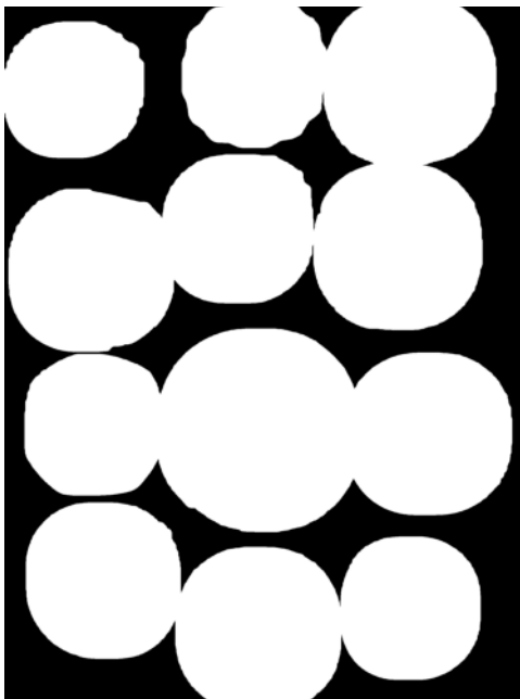
Watershed
