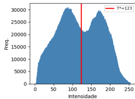
Hist T^*=123
