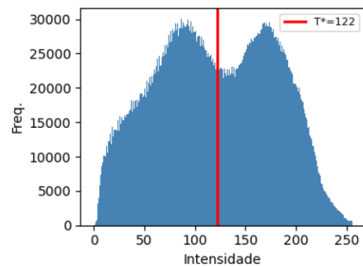
Hist T^*=122
