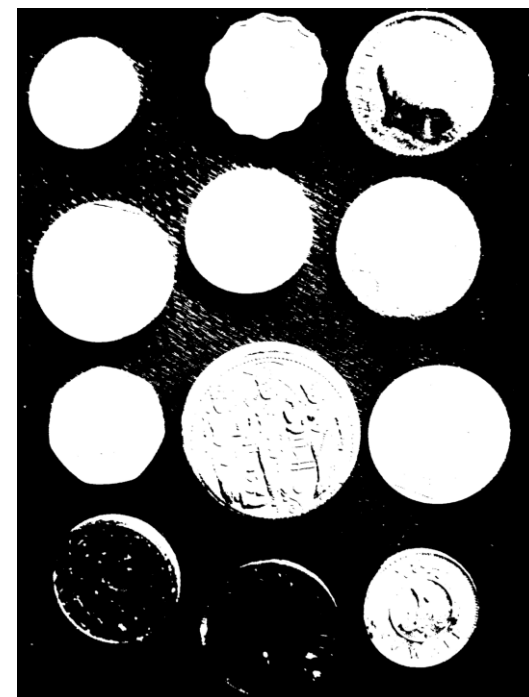
Otsu T^*=122
