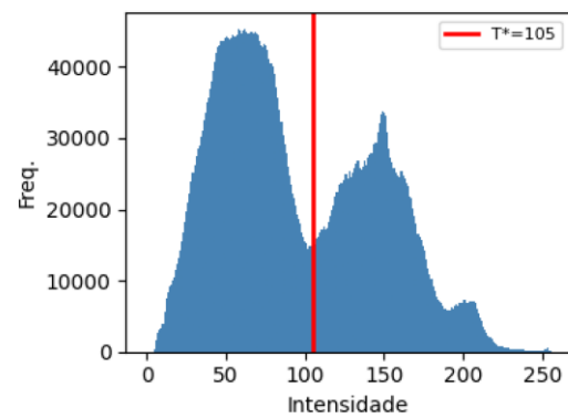
Hist T^*=105
