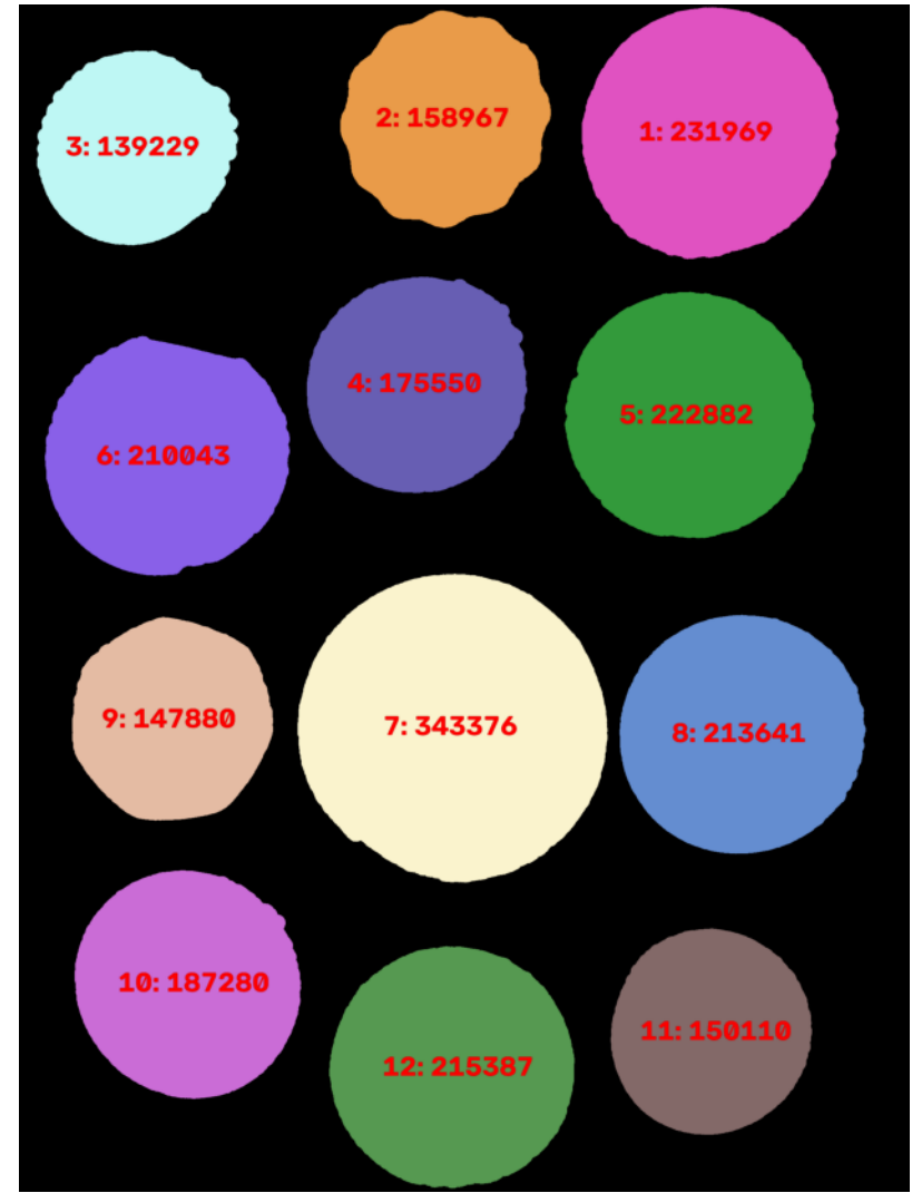
Annotated Areas
