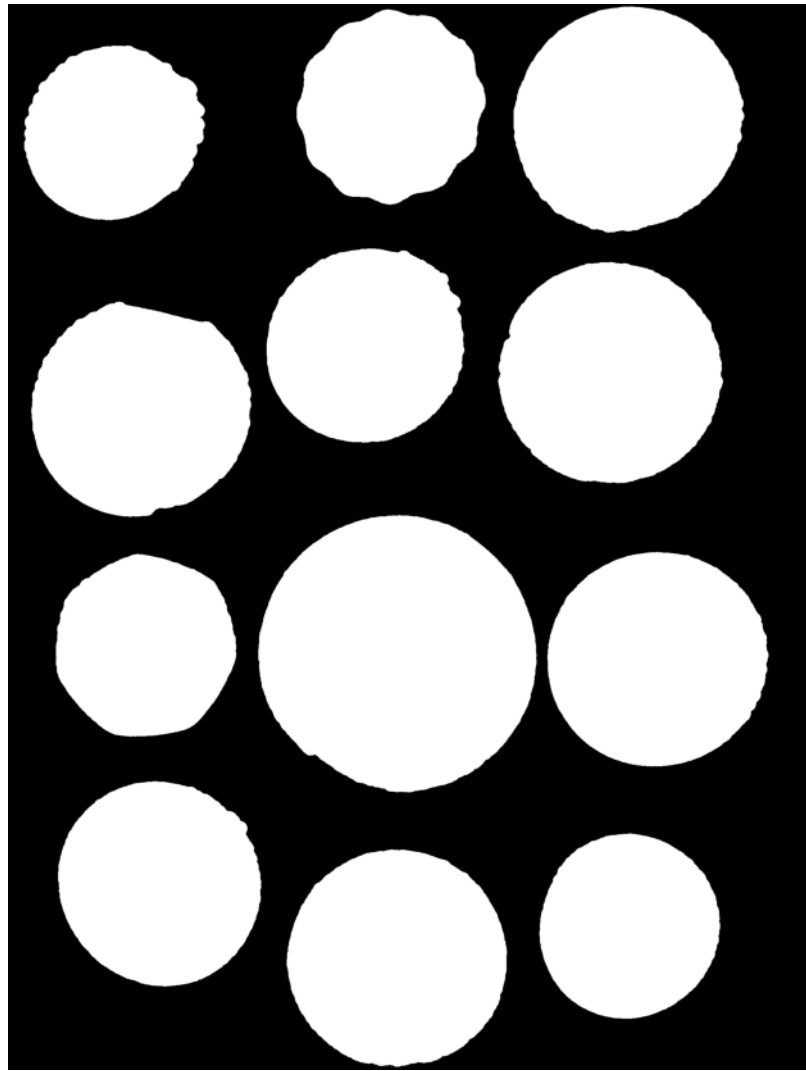
Final Segmentation
