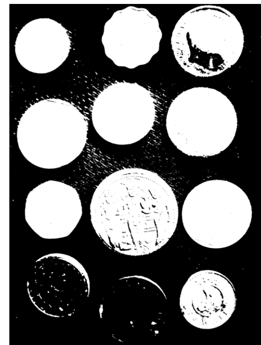
Otsu T^*=122
