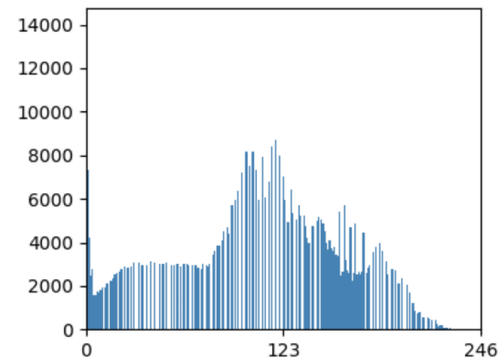
Histogram — result
