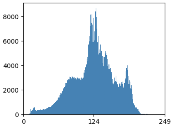
Histogram — Mandrill
