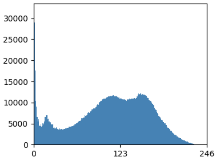
Histogram — Leopard
