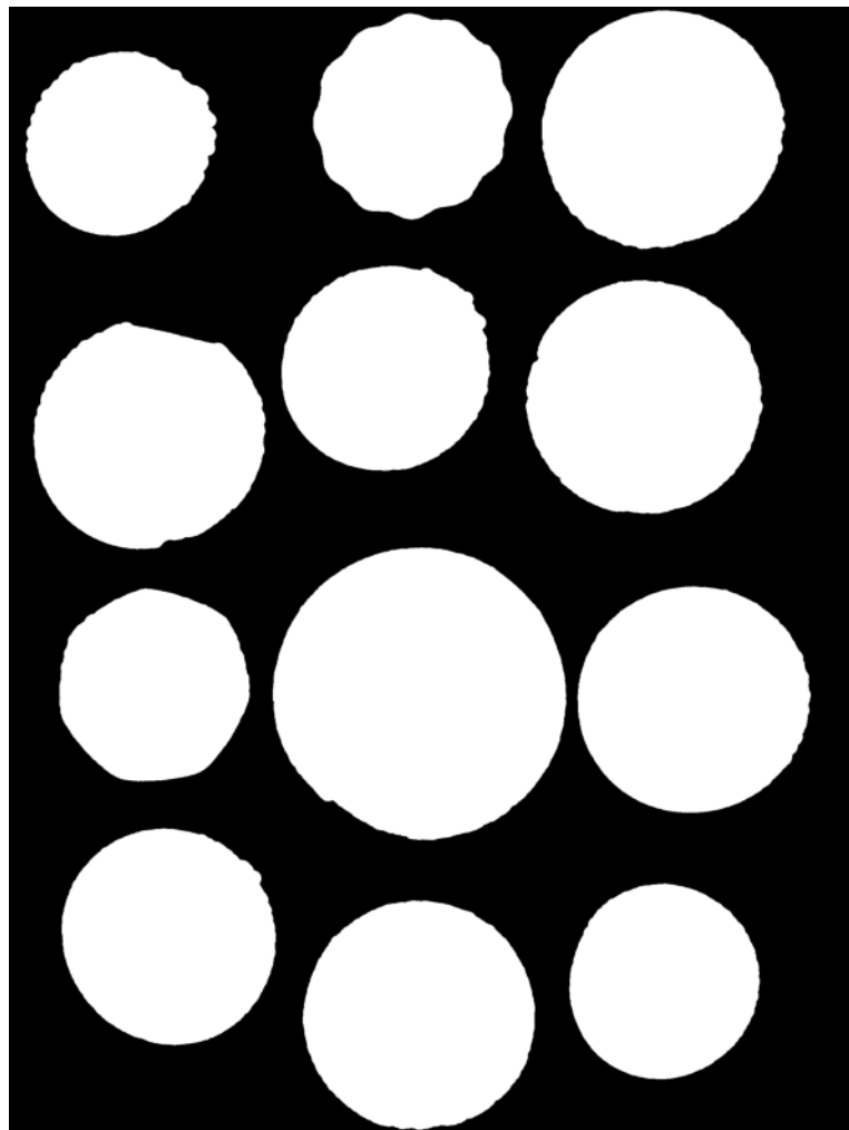
Final Segmentation
