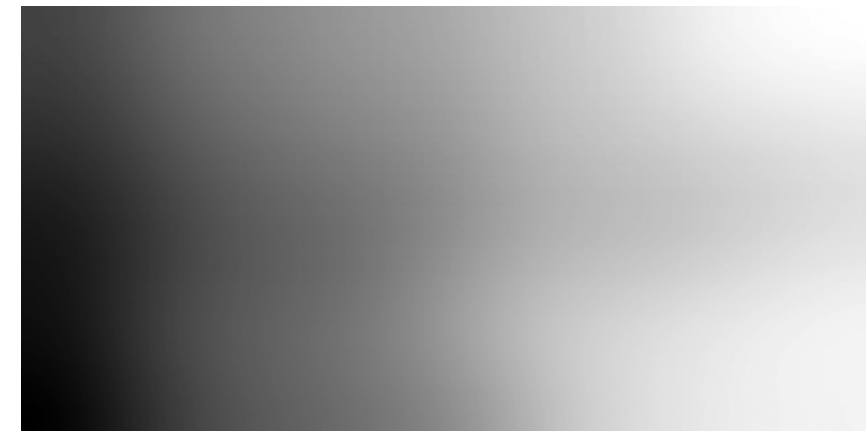
(c) Gaussian
