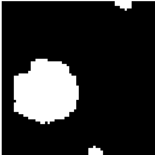
Classical Prediction
