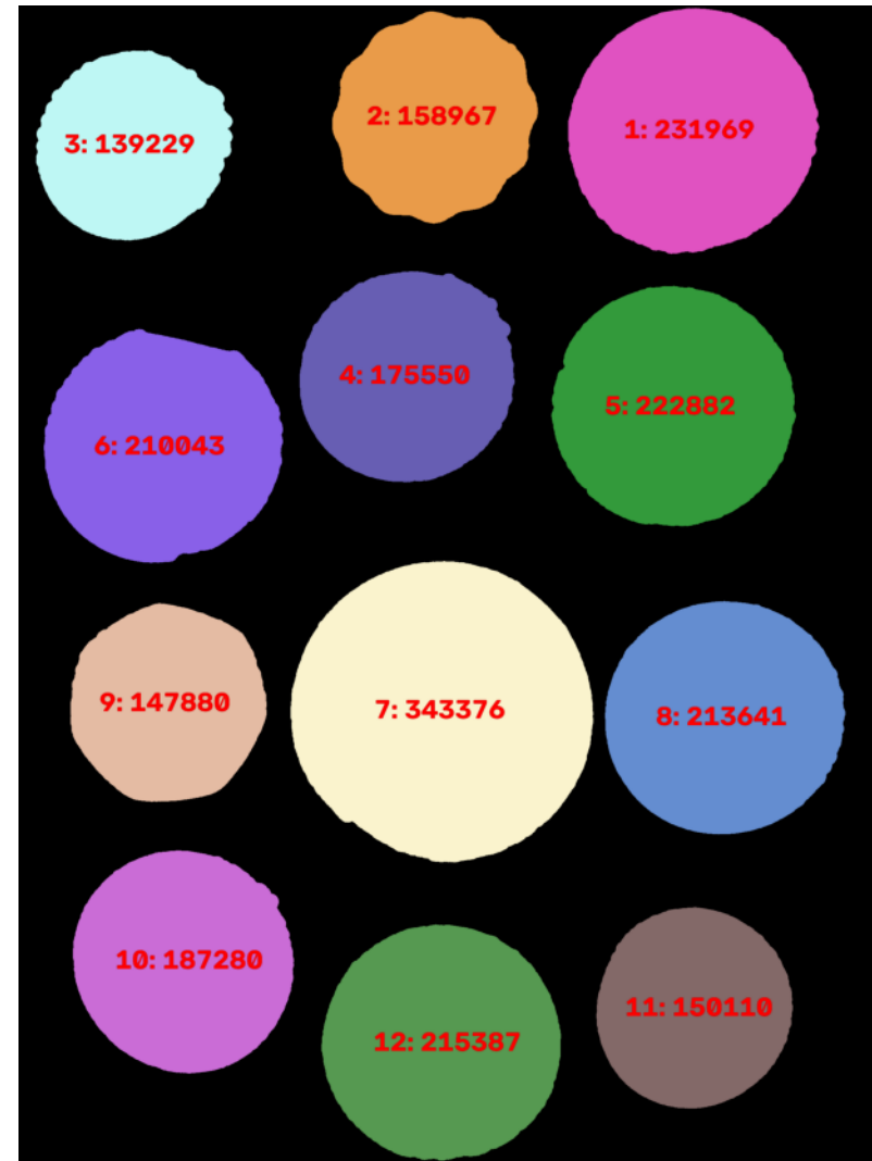
Aree Annotate
