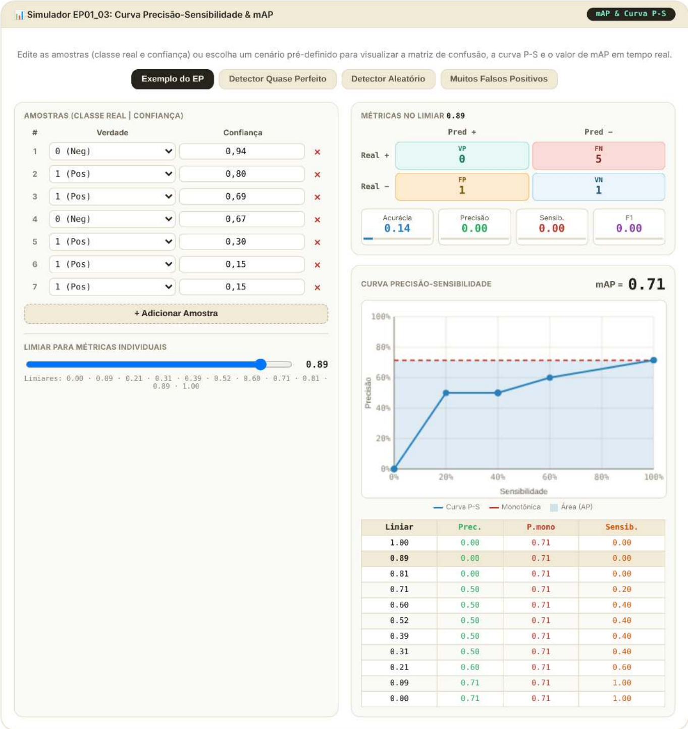
Figura 1.14: Simulador EP01_03: Mean Average Precision (mAP) e Curva P-S
