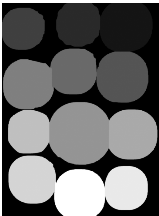
Watershed
