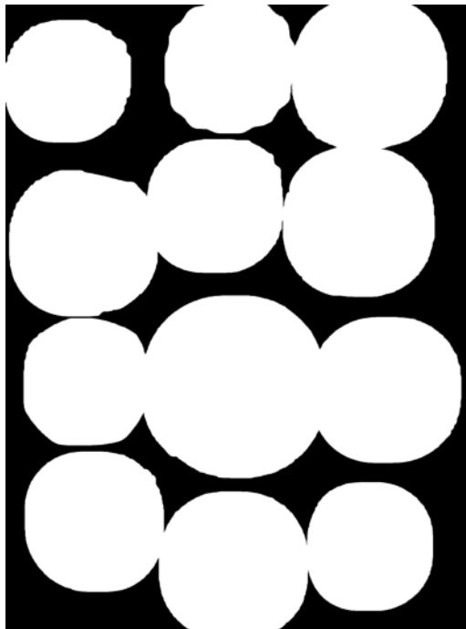
Watershed
