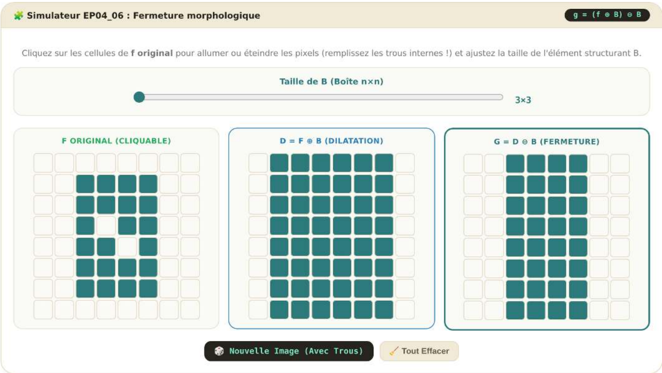
Figure 4.35: Simulateur EP04_06: Fermeture morphologique ( g = (f \oplus B) \ominus B )
