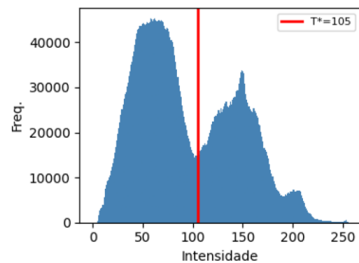
Hist T^*=105
