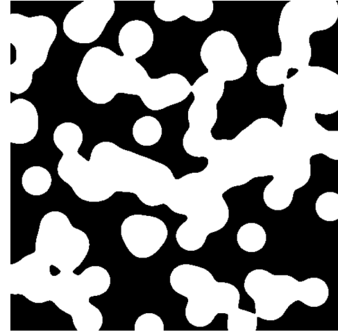
binary_blobs
