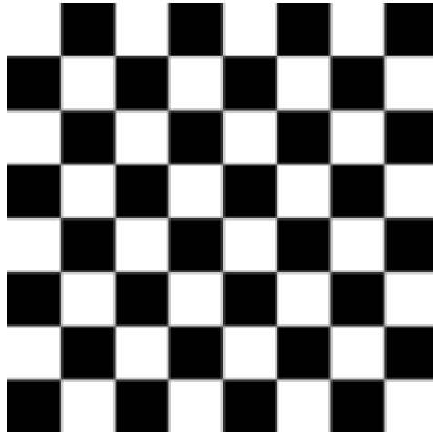
checkerboard
