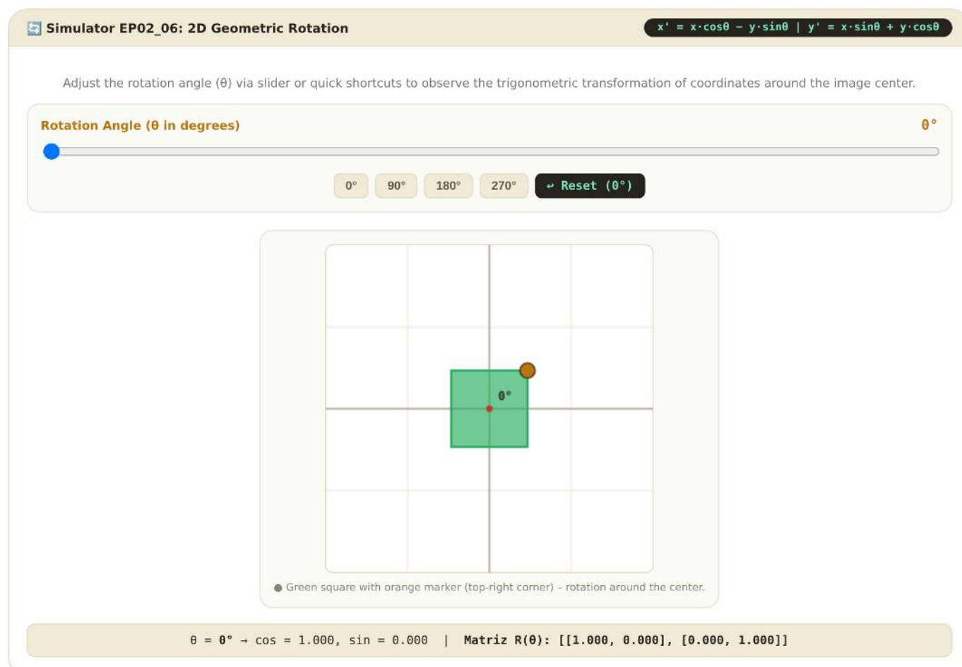
Figure 2.17: EP02_06 Simulator: Image Rotation Around Origin by Angle
